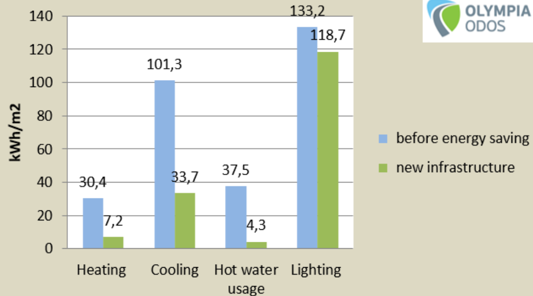
Energy consumption Fuel Station Psathopyrgos
